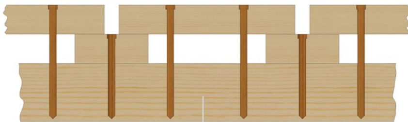
Fassade in Boden- Deckel-Schalung
